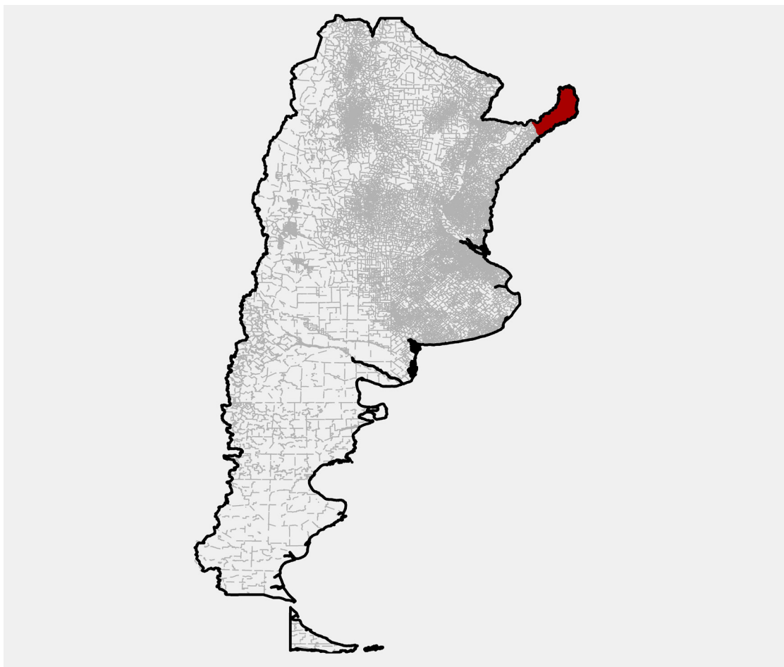
ADM 4/0 boundaries for all of Argentina; area in red, over Misiones Province, is available as sample data
